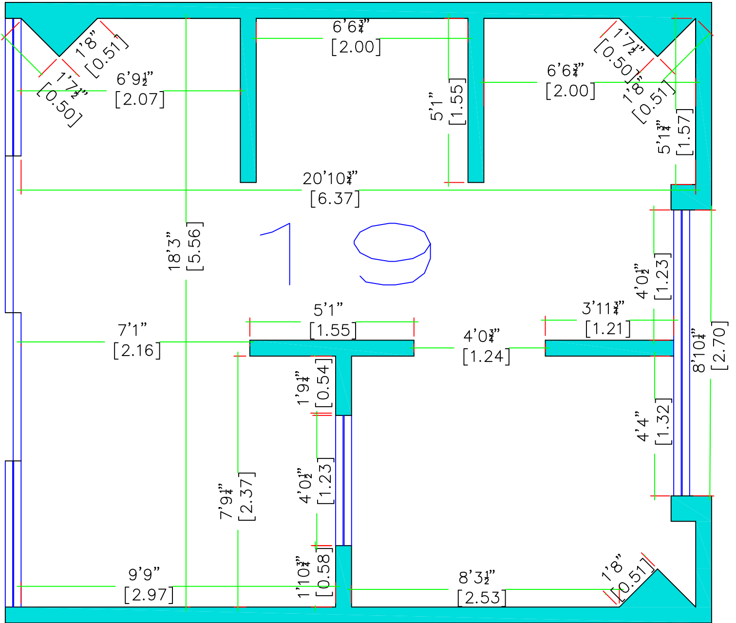
ARCHITECTURAL PLAN L-19 PLAZA "B" MEASUREMENTS
