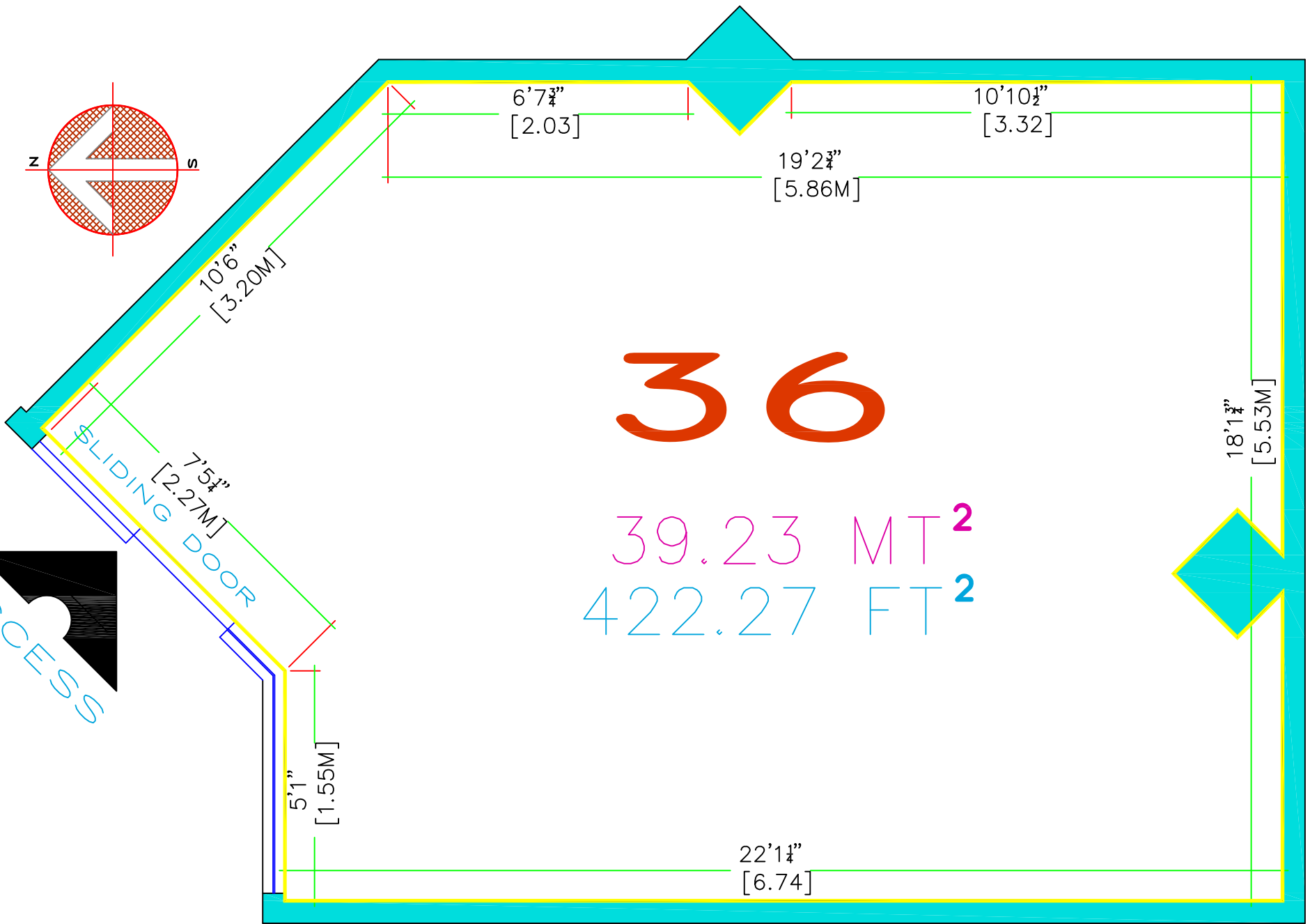
ARCHITECTURAL PLAN L-36 PLAZA "A" MEASUREMENTS
