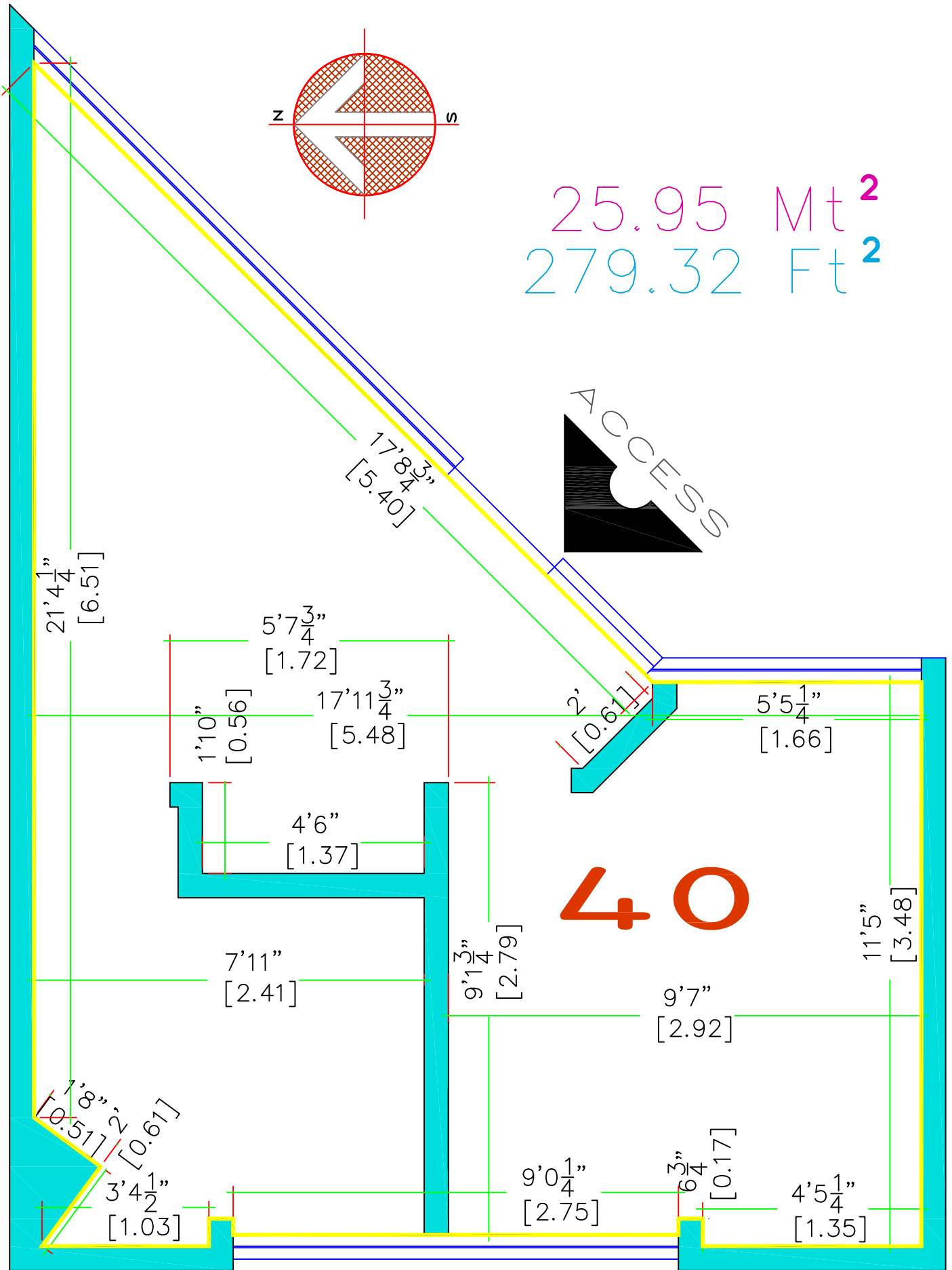
ARCHITECTURAL PLAN L-40 PLAZA "A" MEASUREMENTS
